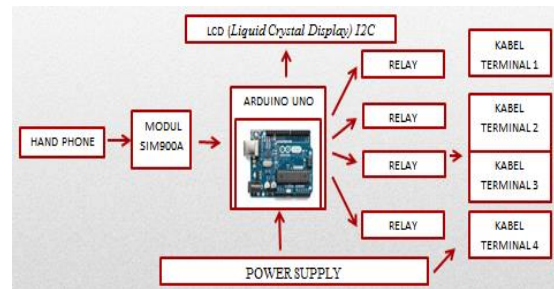
Gambar 1 Blok diagram terminal stop kontak otomatis
